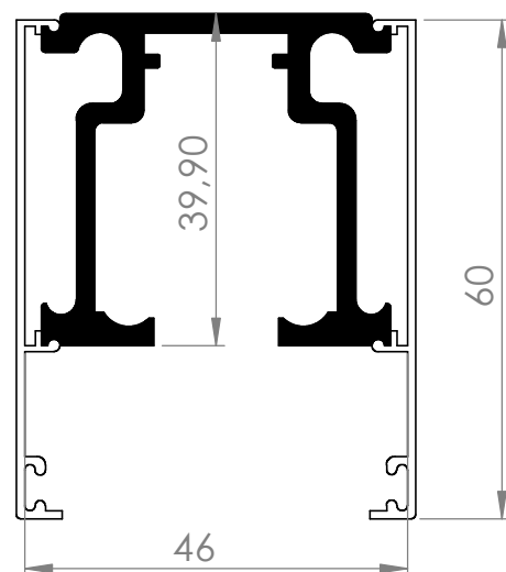
P125 Ceiling mounted
