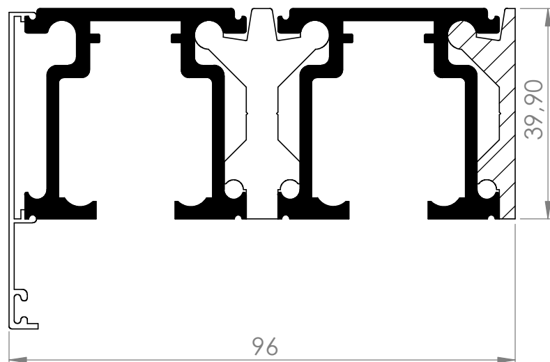
P125 Double Track stacking system wall mounted
