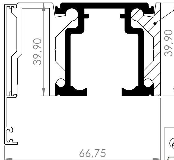
P125 Track + Fix glass 10-12 mm
